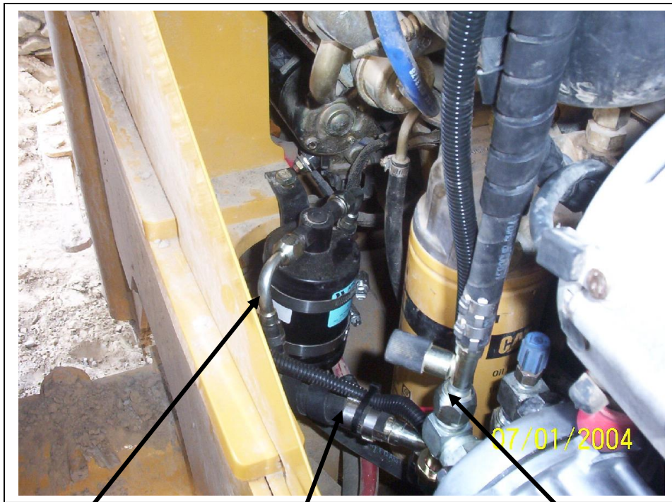
5/16" hose from the condenser
